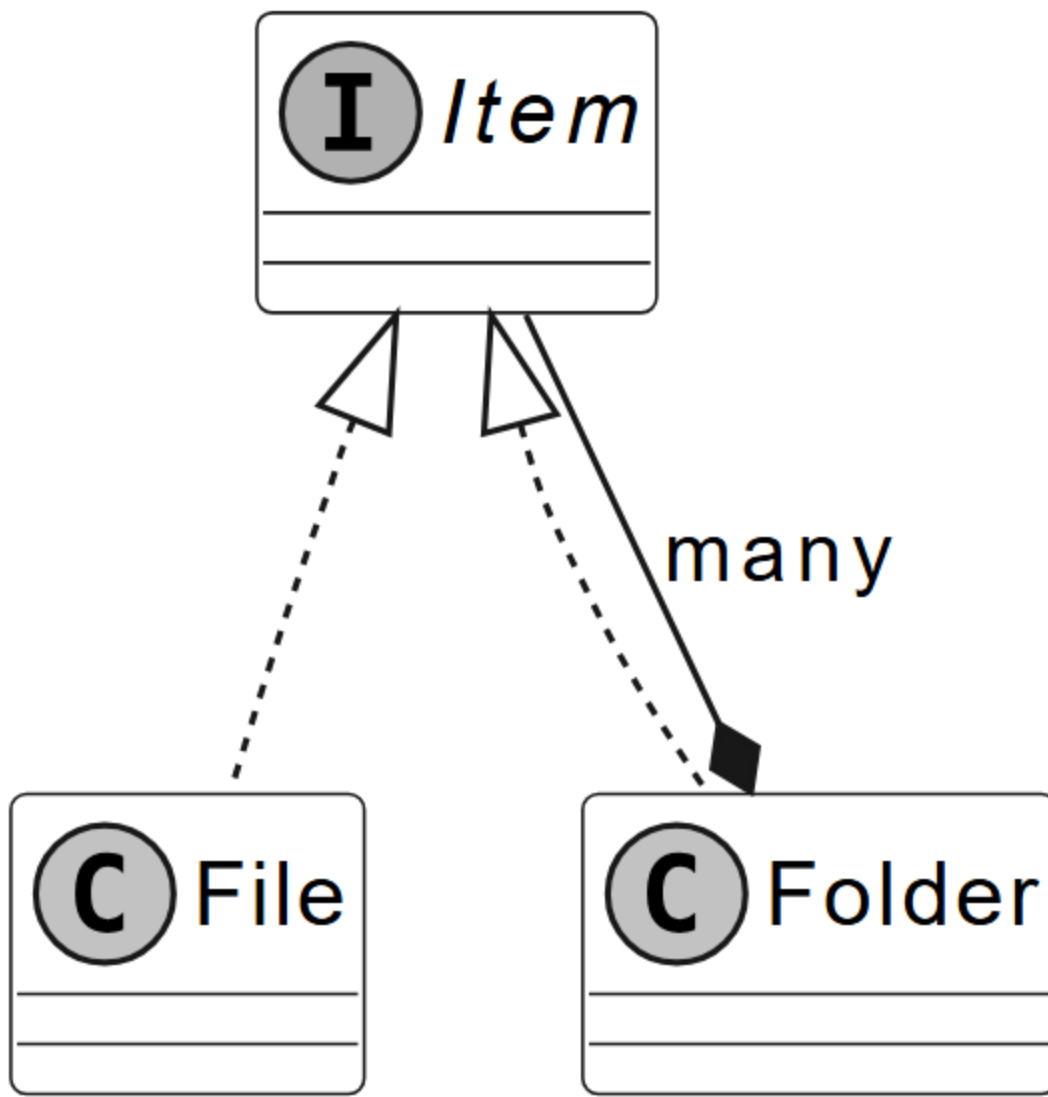
Item interface and concrete classes
