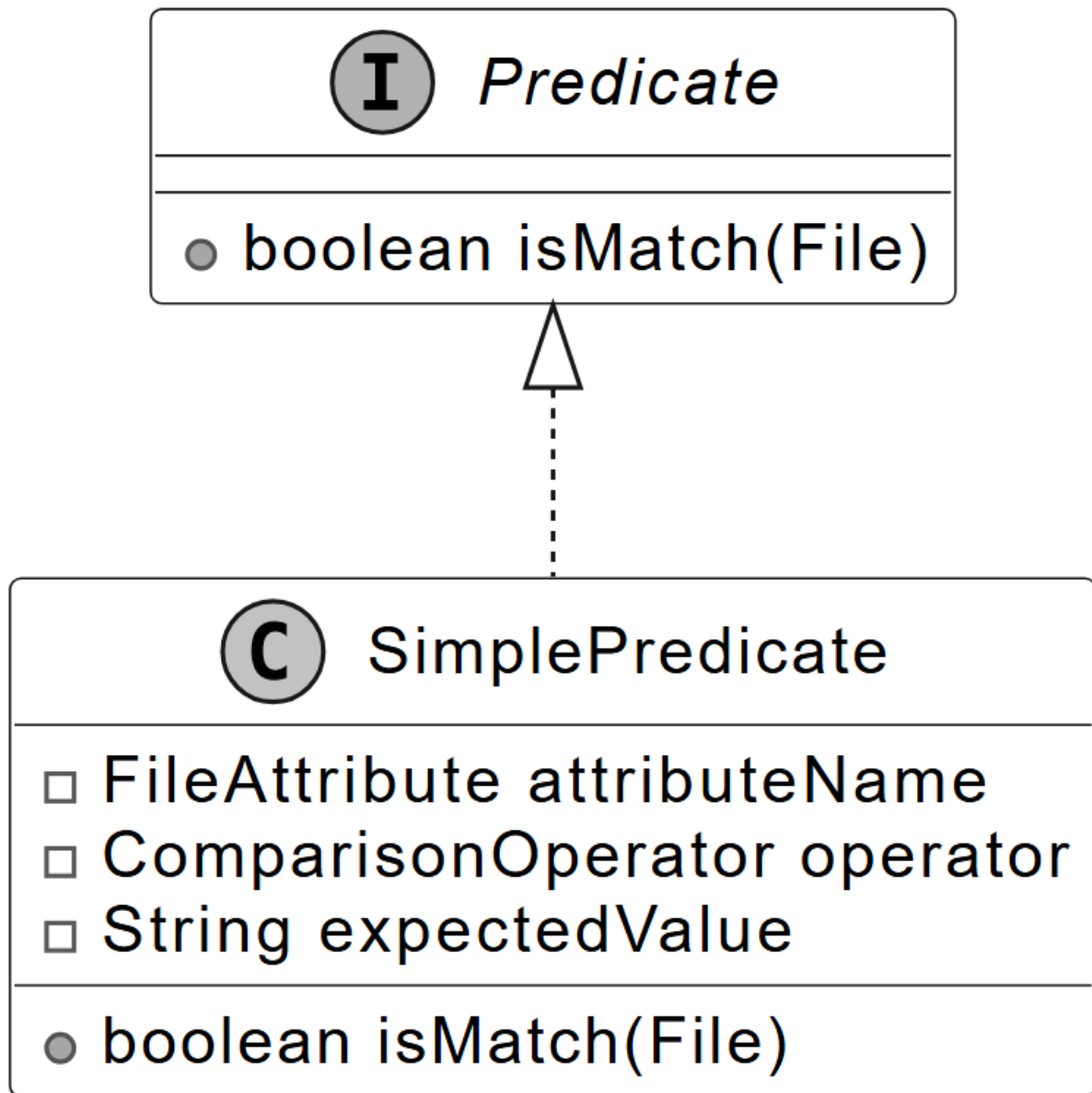
Predicate interface and concrete class
